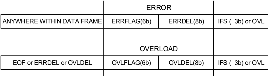
Figure 38-12. Error and Overload Frame
