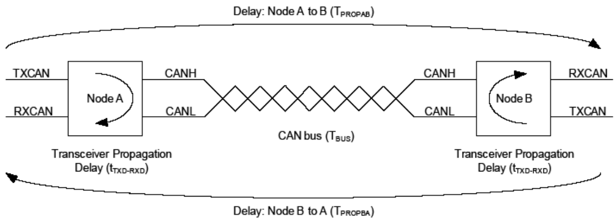
Figure 38-4. Propagation Delay
