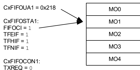
Figure 38-23. FIFO 1 - FIFO Fully Transmitted
