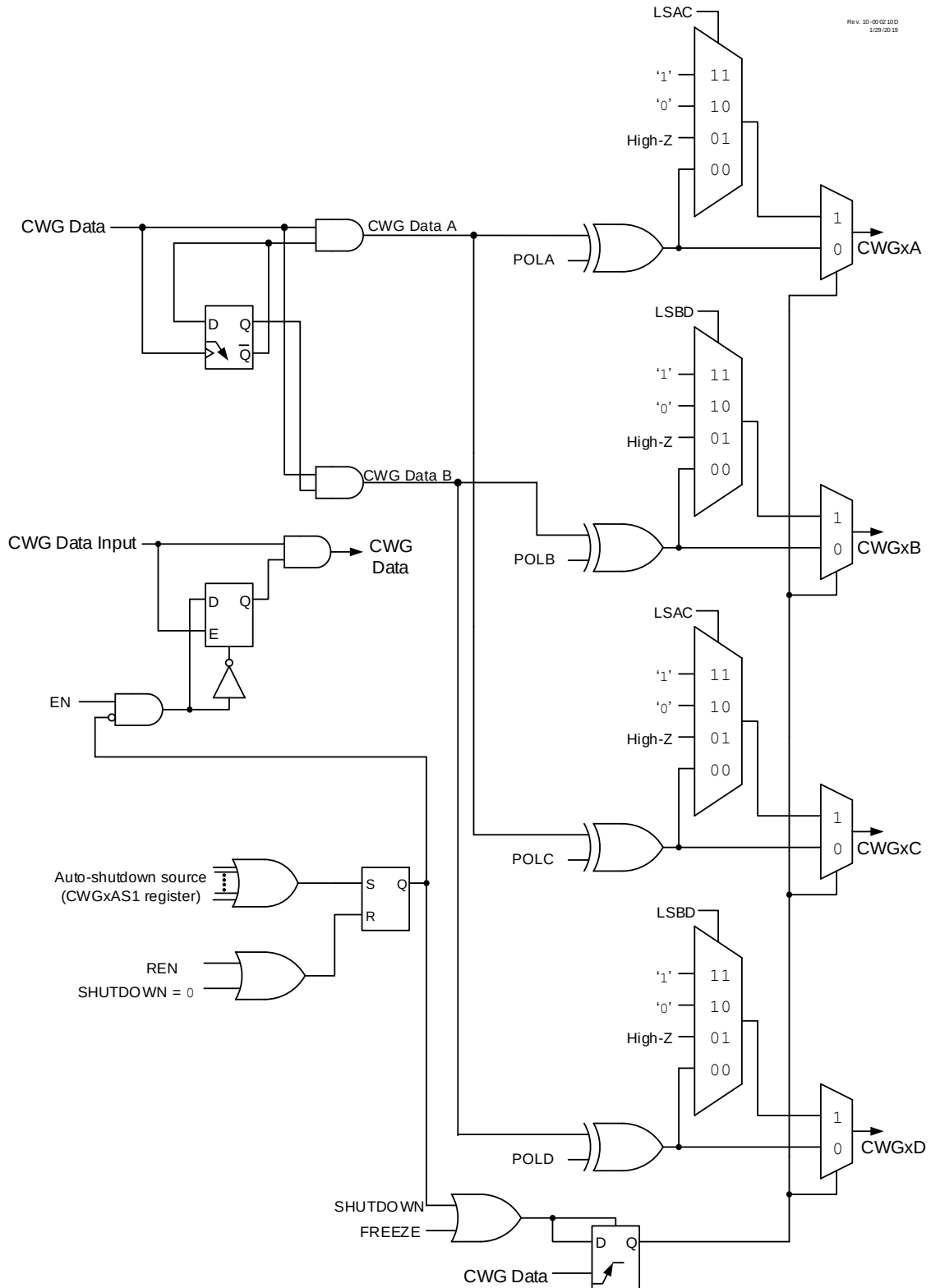
Figure 32-4. Simplified CWG Block Diagram (Push-Pull Mode, MODE = 'b101)
