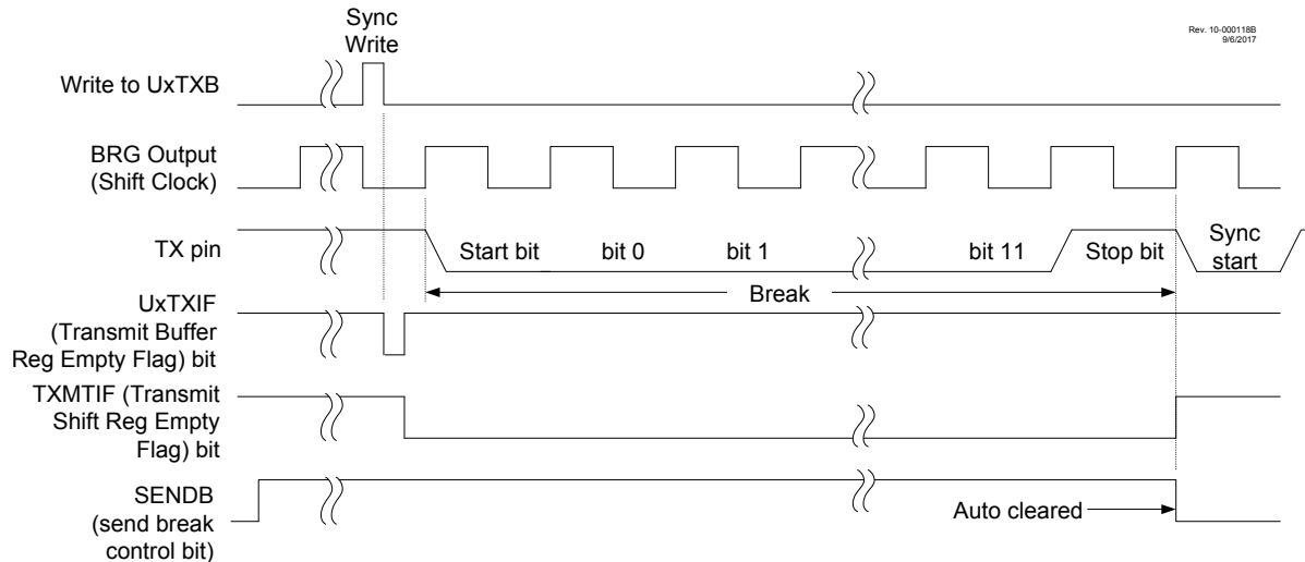
Figure 35-15. Send-Break Sequence
