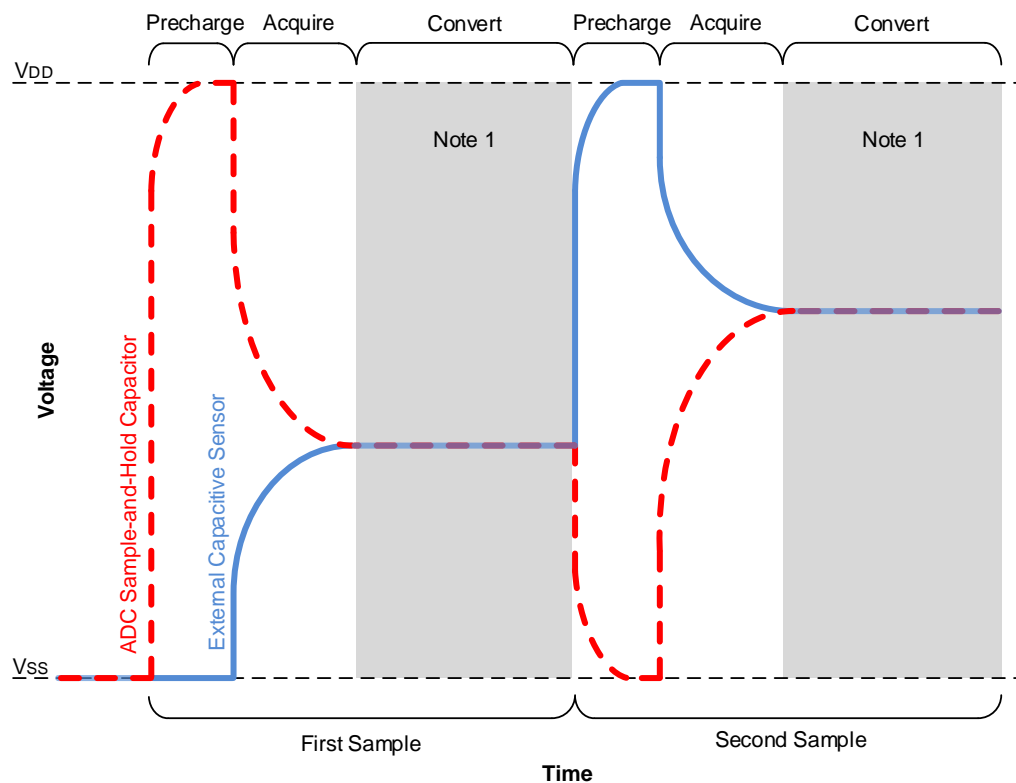
Figure 41-8. Differential CVD Measurement Waveform
