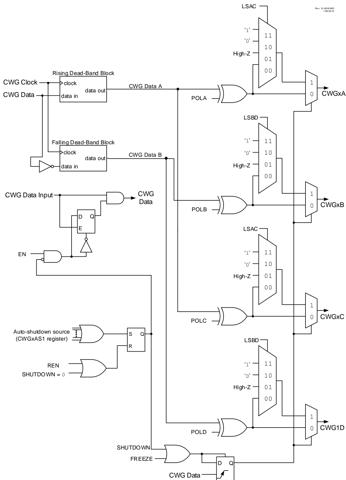
Figure 31-2. Simplified CWG Block Diagram (Half Bridge Mode, MODE = 'b100)
