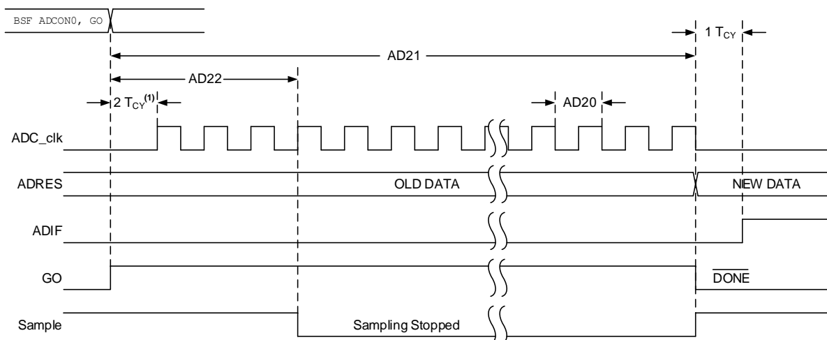
Figure 47-10. ADC Conversion Timing (ADC Clock from ADCRC)
