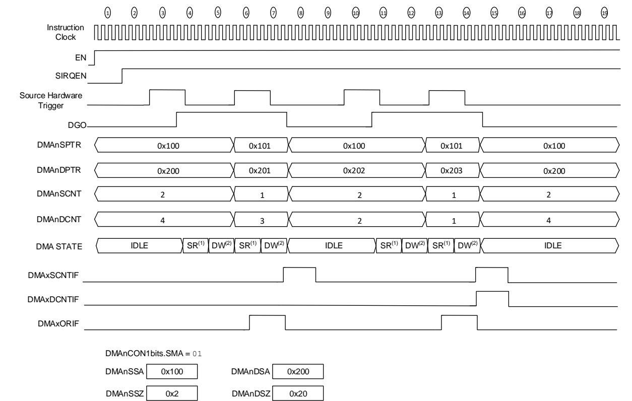
Figure 16-10. Overrun Interrupt
