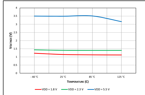
FIGURE 40-94: Typical Input High Voltage with I²C Level.
