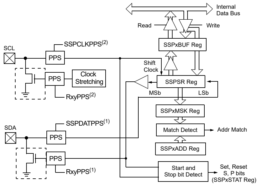
FIGURE 33-3: MSSP BLOCK DIAGRAM (I 2 C CLIENT MODE)
