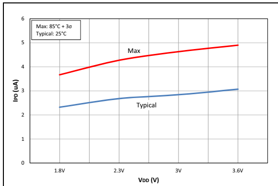
FIGURE 40-27: I PD , 3V Pump Output (NP), PIC16LF19195/6/7 Only.
