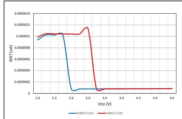
FIGURE 40-28: Typical I BAT .
