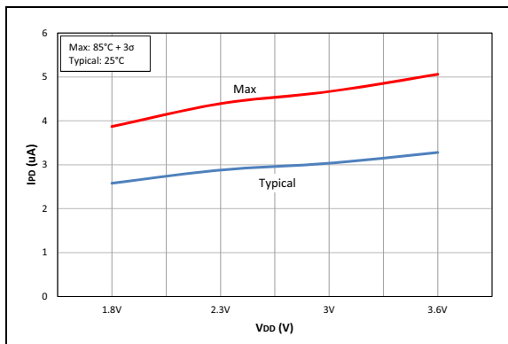
FIGURE 40-26: I PD , 3V Pump Output (LP), PIC16LF19195/6/7 Only.
