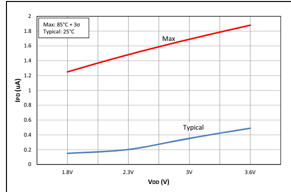
FIGURE 40-16: IPD, Base, LP mode, PIC16LF19195/6/7 Only.
