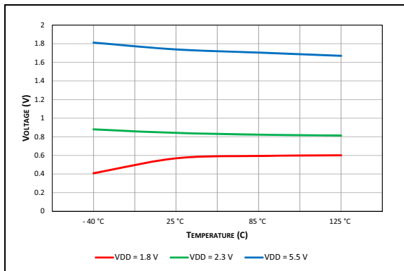
FIGURE 40-93: Typical Input Low Voltage with I²C Level.
