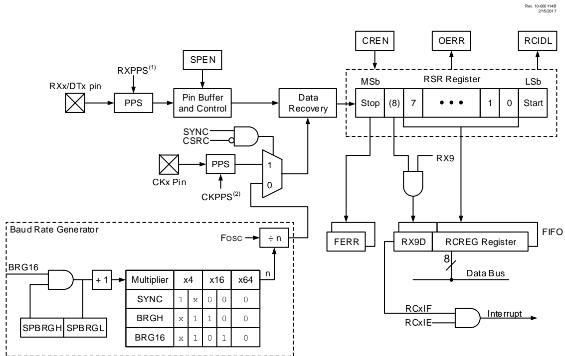
Figure 28-2. EUSART Receive Block Diagram
