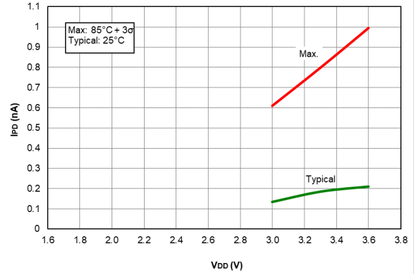
Figure 40-10. I_{PD} Comparator PIC16F18424/44 only
