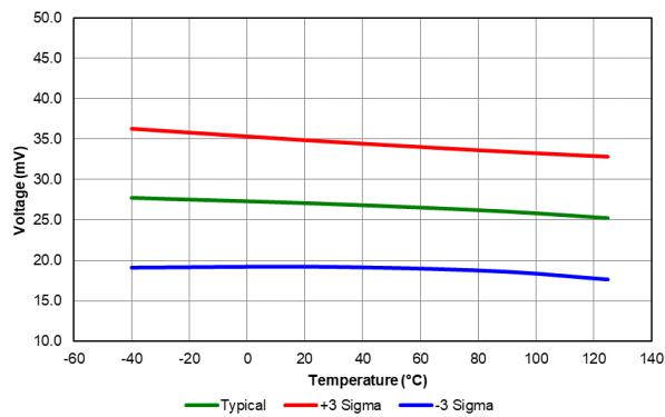
Figure 40-45. LPBOR Reset Hysteresis, All devices
