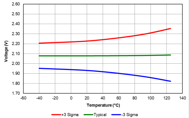
Figure 40-44. LPBOR Reset Voltage, All devices
