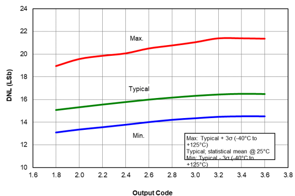
Figure 40-72. DAC DNL Error, VDD = 3.0V, PIC16LF18424/44 only
