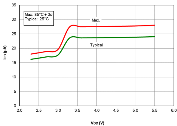
Figure 40-11. I_{PD} Base, 01 PIC16F18424/44 only
