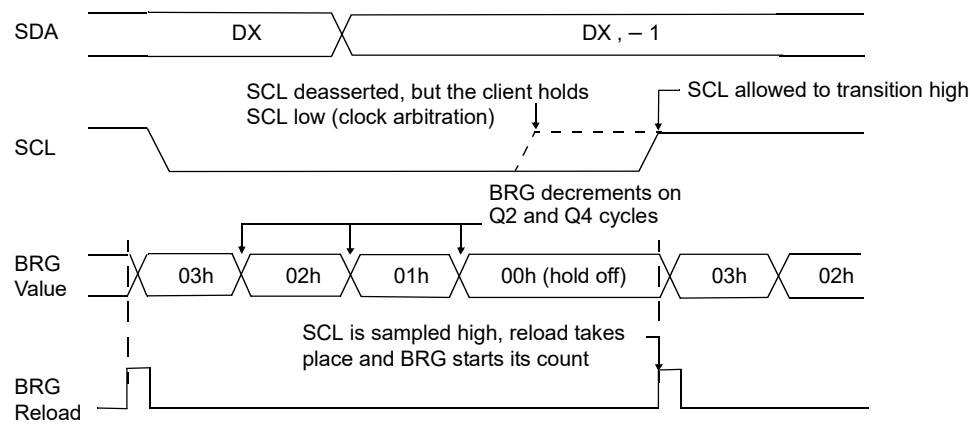
Figure 29-25. Baud Rate Generator Timing with Clock Arbitration
