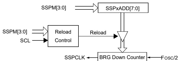
Figure 29-40. Baud Rate Generator Block Diagram
