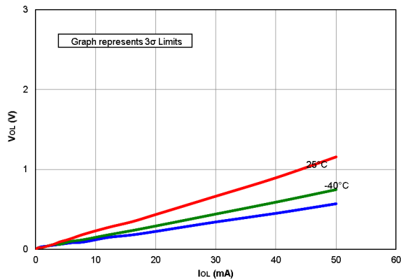
Figure 40-33. VOL vs. IOL Overtemperature, VDD = 5.5V, PIC16F18424/44 only
