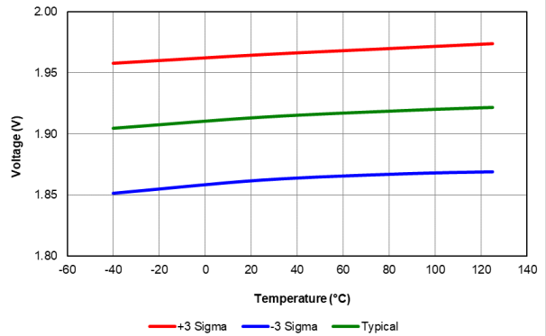
Figure 40-42. Brown-Out Reset Voltage, Trip Point BORV = 01, PIC16F18424/44 only
