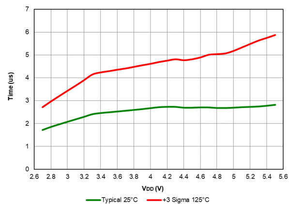
Figure 40-47. BOR Response Time, PIC16F18424/44 only
