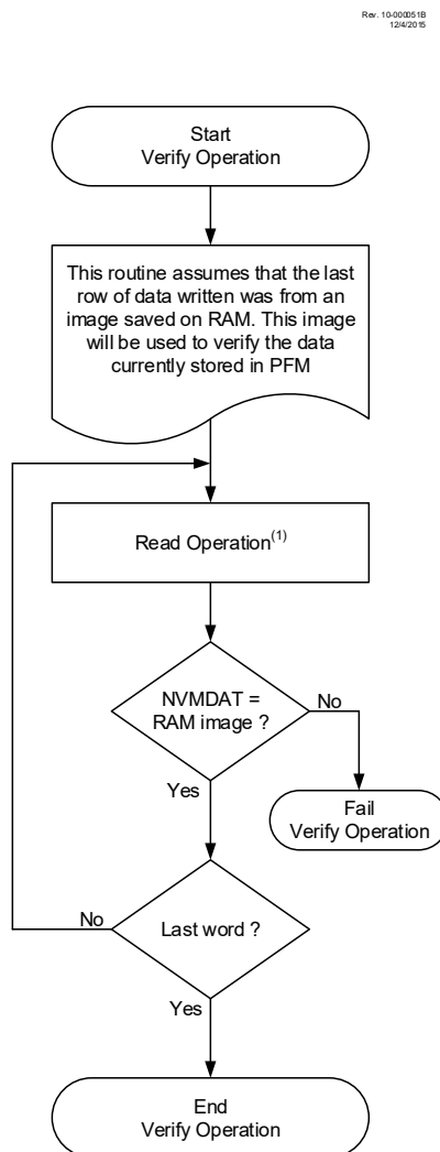
Figure 6-7. Flash Program Memory Verify Flowchart
