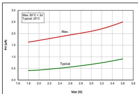
FIGURE 37-29: I_{PD} , Watchdog Timer (WDT), PIC16LF1764/5/8/9 Only.
