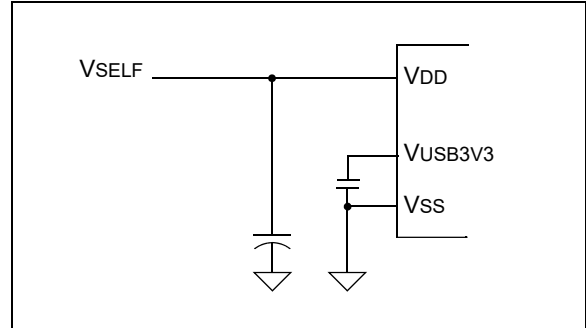
FIGURE 26-9: SELF-POWER ONLY
