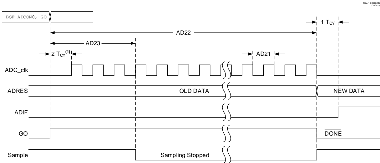
Figure 32-10. ADC Conversion Timing (ADC Clock from F_{RC} )
