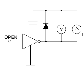
Figure 8 V_F Test Circuit
