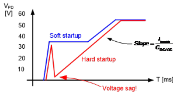
Figure 6-1. Comparison of Input Voltages without Soft-start (Hard Startup) and Soft-start (Soft Startup)
