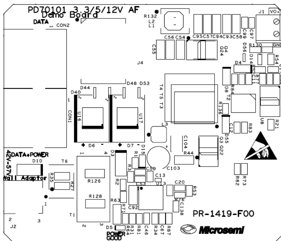
Figure 26: Top Silk
