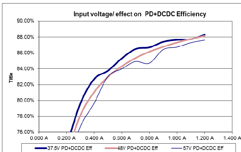
Figure 24: PD70101EVB15F12 PD+DCDC Efficiency for 3 Vin Values
