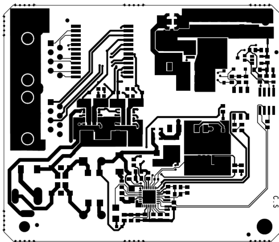
Figure 27: Top Layer
