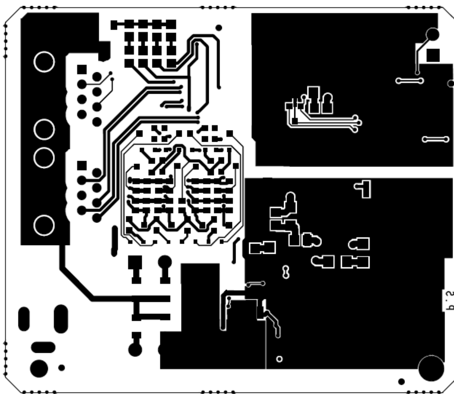
Figure 28: Bottom Layer
