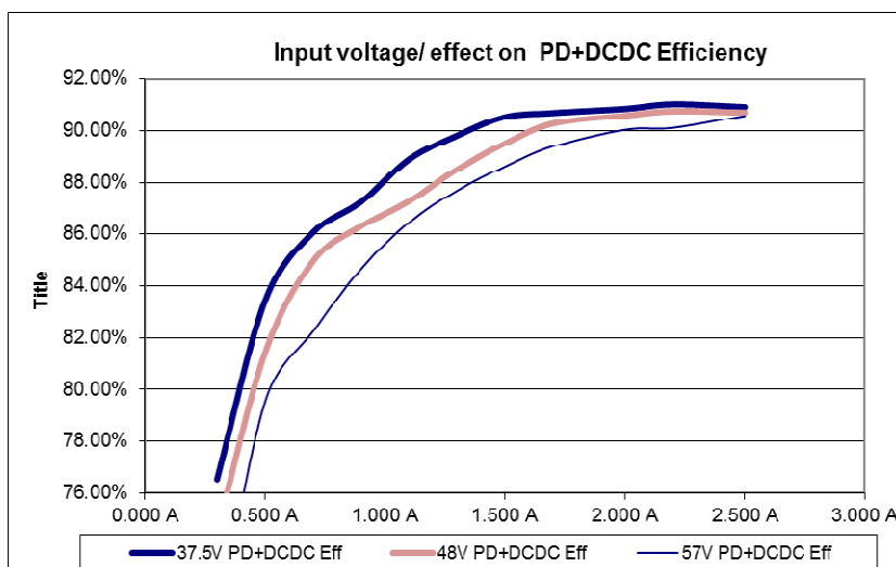
Figure 19: PD70101EVB15F5 PD+DCDC Efficiency for 3 Vin Values
