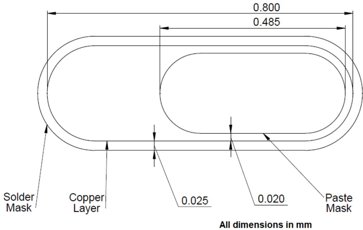
Figure 3-5. Pin Geometry
