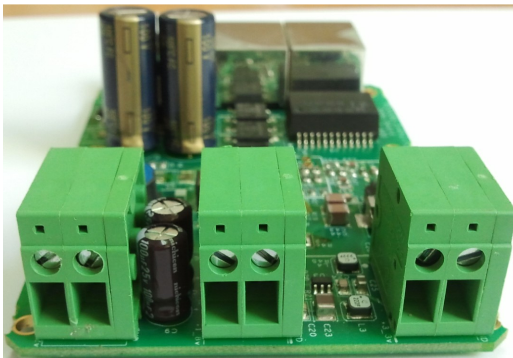
Figure 4: Vout Connectors
