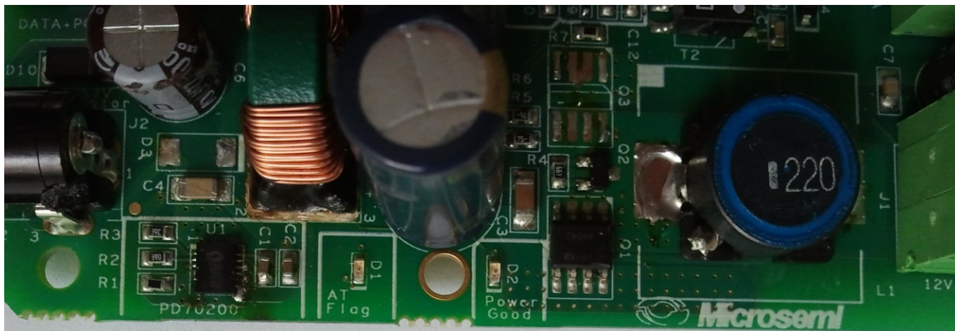
Figure 5: Powr_Good LED Indication
