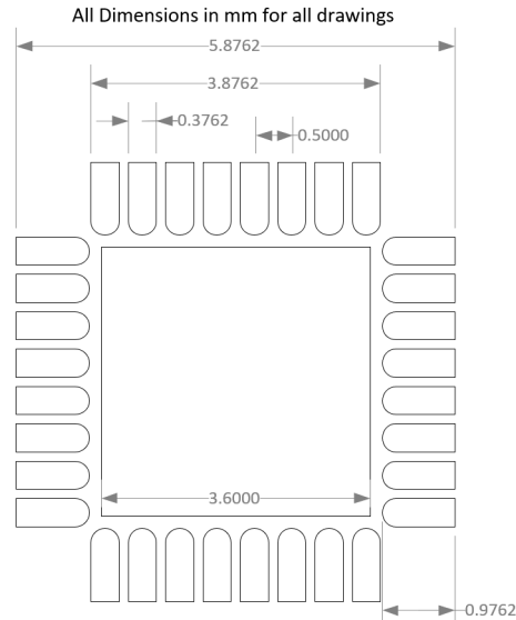
Figure 4-3. PD69210 and PD69220 Solder Mask
