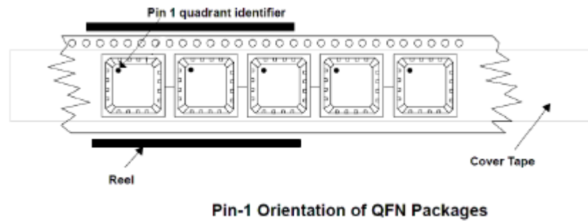
Figure 18 • PD69208T4 Tape and Reel Pin-1 Orientation
