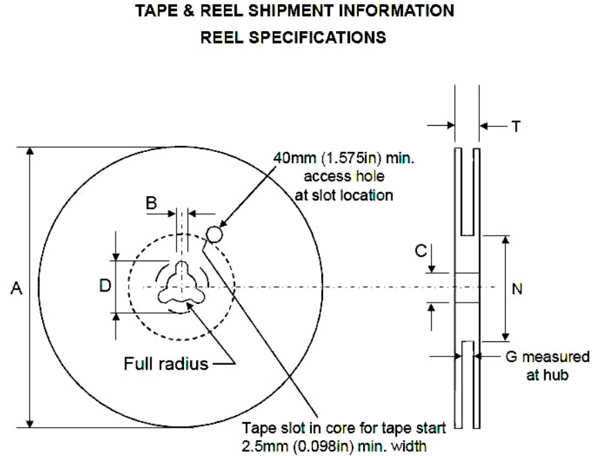
Figure 20 • PD69208M Reel Specifications
