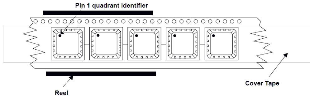
Figure 5-9. Tape Specifications
