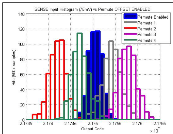
FIGURE 4-4: Illustration of the Four Permute Combinations that the ADC Cycles through and the Resulting Low Average Offset. Each Bin Represents One Code.
