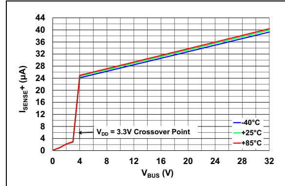
FIGURE 2-6: I_{SENSE+} Input Current vs. Common-Mode Voltage ( V_{BUS} ) Integrate State ( V_{DD} = 3.3\text{V} , V_{SENSE} = 100\text{ mV} ).
