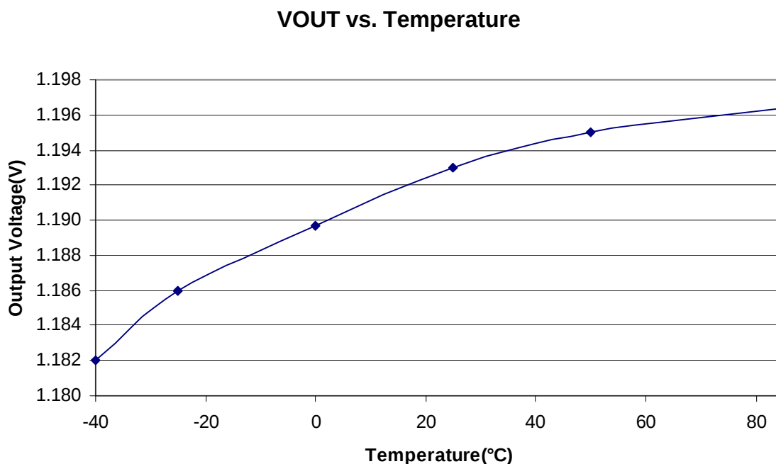
Figure 4 - Output voltage vs temperature(VIN=5V, NO LOAD)
