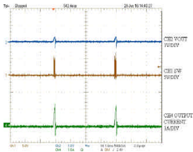
Figure 11 - Output Short
