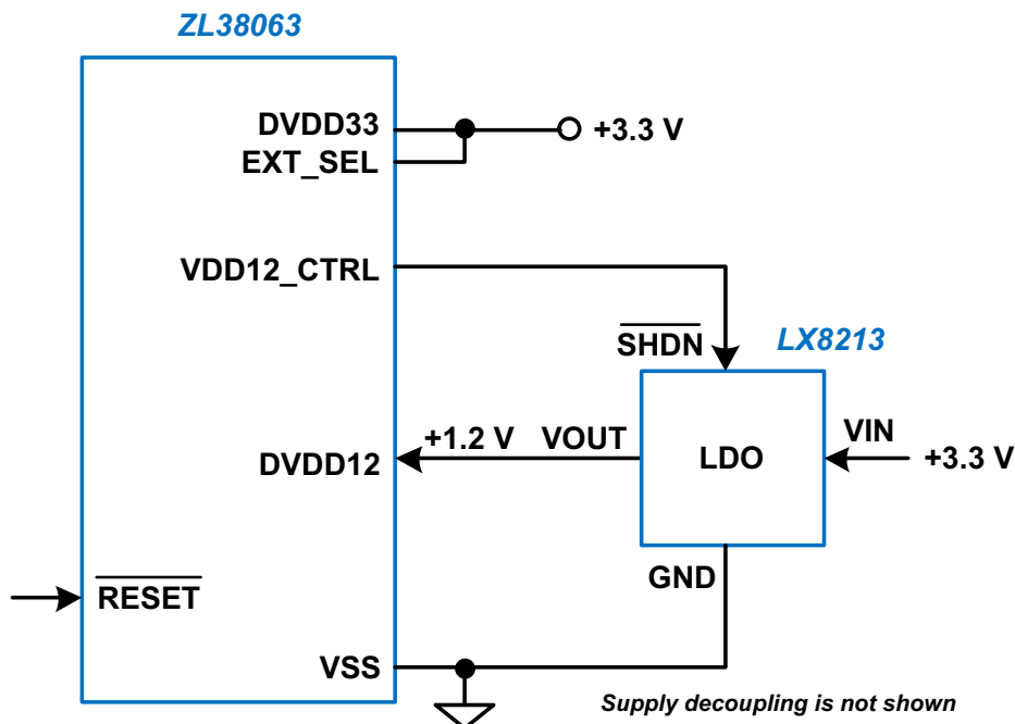
Figure 24 • External +1.2 V Power Supply Configuration
