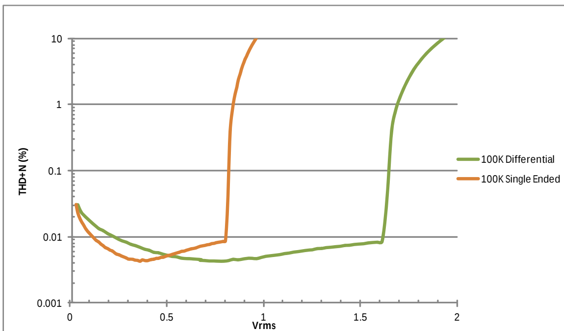
Figure 30 • THD+N Ratio versus V_{RMS} – Driving High Impedance
