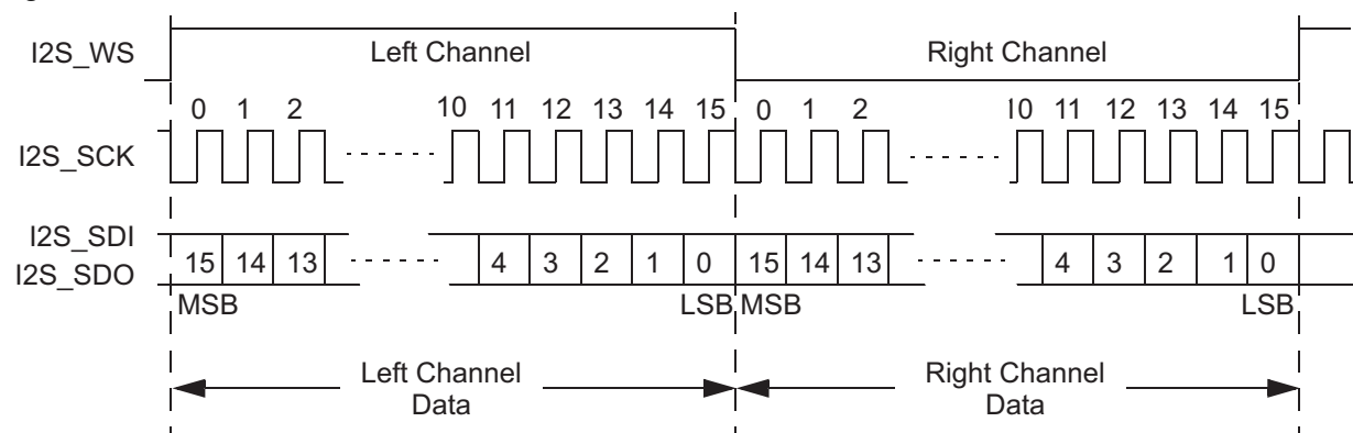
Figure 8 • Left Justified Mode
