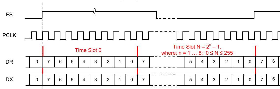
Figure 15 • TDM – GCI Master Functional Timing Diagram
