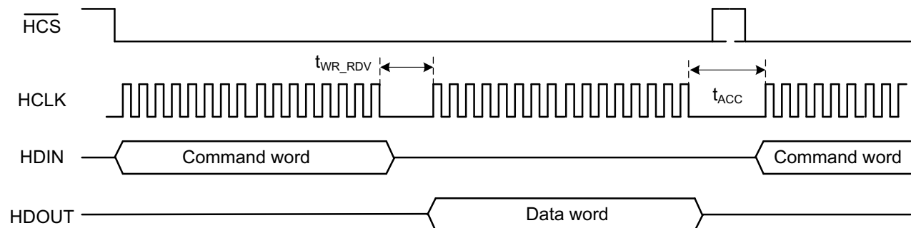
Figure 21 • SPI Slave Command Framing Mode – Read
