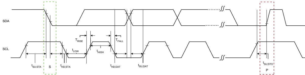
Figure 21 • I²C Timing Parameter Definition
