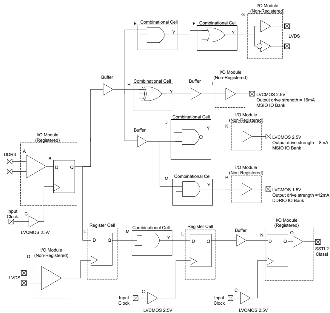
Figure 2 • Timing Model
