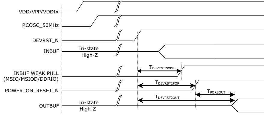
Figure 20 • DEVRST_N to Functional Timing Diagram when MSS/HPMS is not used
