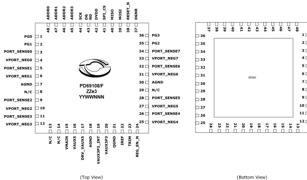
Figure 5 • PD69108/F Pinout
