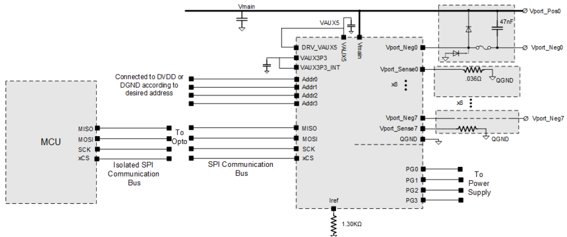
Figure 1 • Typical Application
