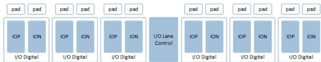
Figure 7 • I/O Topology
