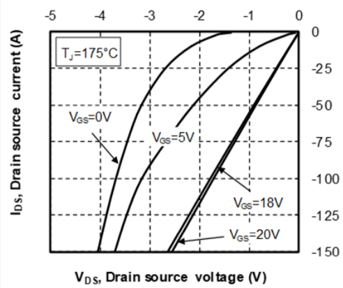
Figure 13 • 3 rd Quadrant Characteristics, T_J = 175^\circ\text{C}
