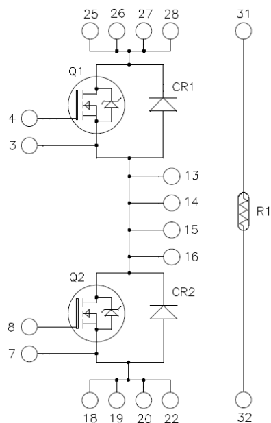
Figure 1 • MSCSM120AM11CT3AG Electrical Schematic
