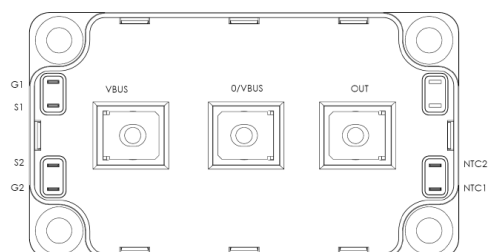
Figure 2 • MSCSM120AM027CT6AG Pinout Location
