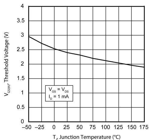
Figure 11 • V_{GS(th)} vs. Junction Temp.
