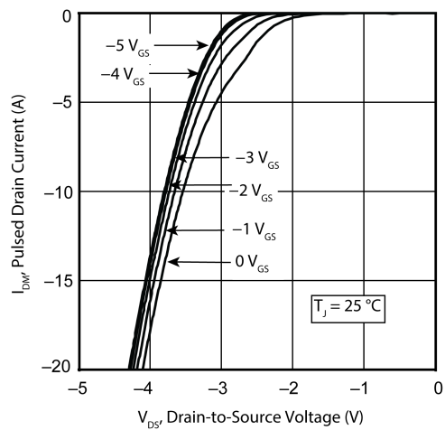
Figure 9 • I_{DM} vs. V_{DS} 3 rd Quadrant Conduction
