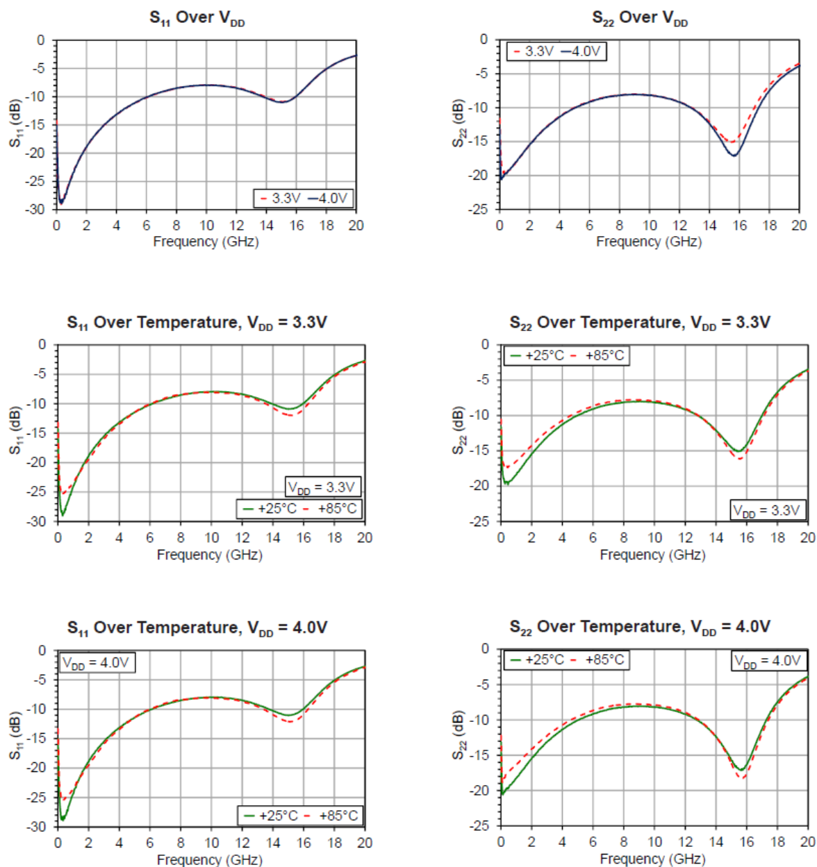
Figure 2 S_{11} and S_{22} over V_{DD} and Temperature
