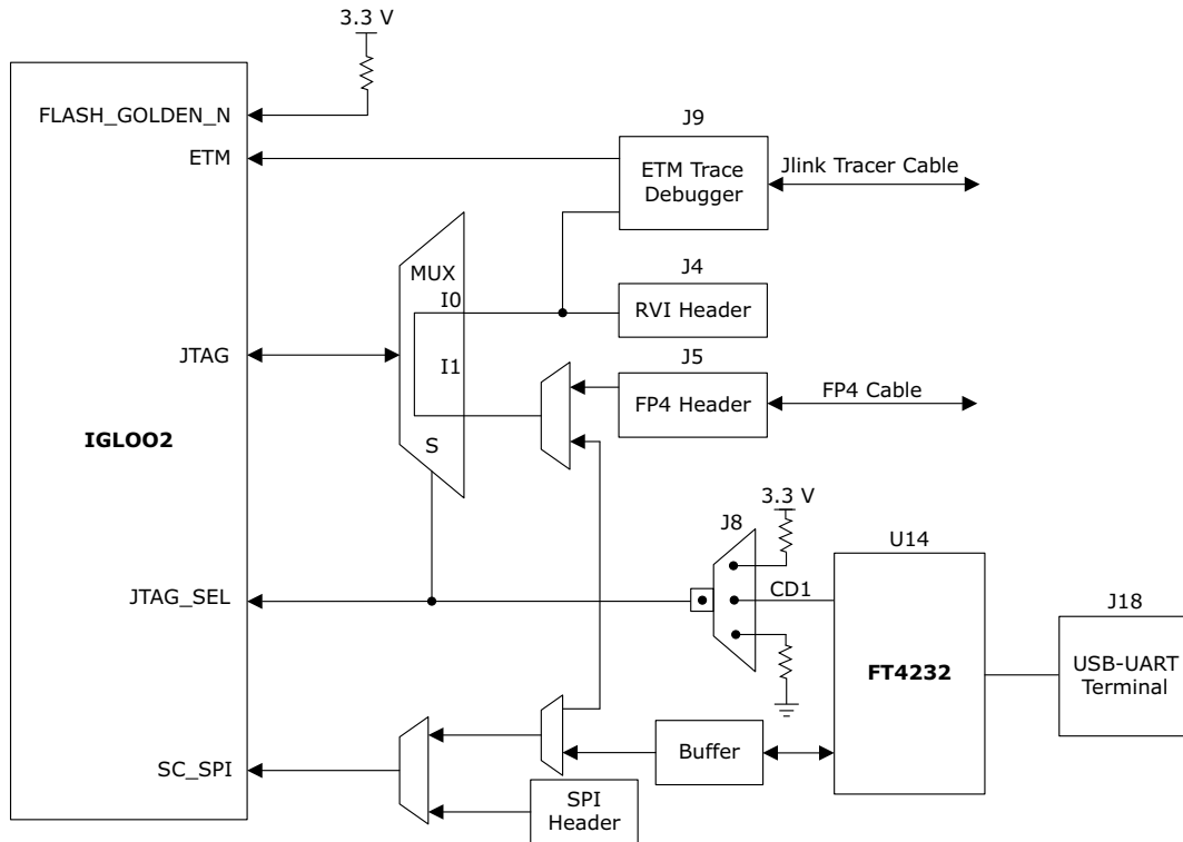
Figure 11 • IGLOO2 Programming Interface
