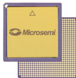
b.s. 1.220x1.220" (31.00x31.00 mm) h. CCGA – 218 mils (5.535 mm) h. LGA – 129 mils (3.28 mm) p. 39 mils (1.00 mm)
