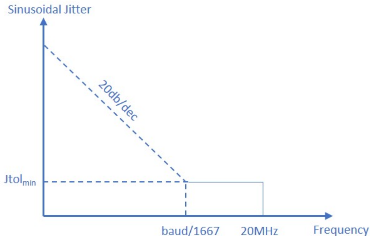
Figure 3 • LVDS Jitter Tolerance Plot
