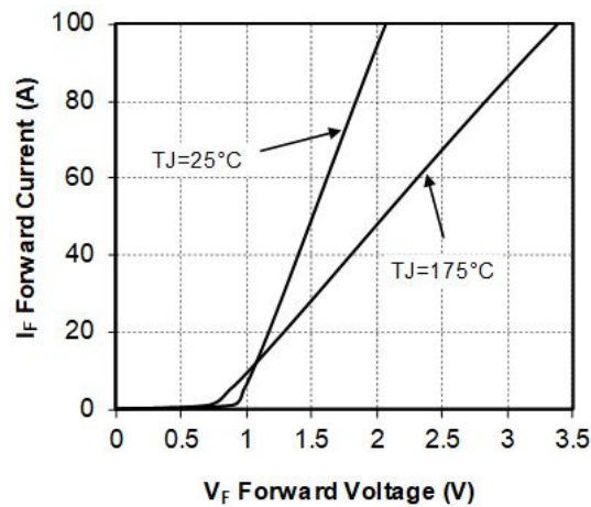
Figure 1-16. Forward Characteristics
