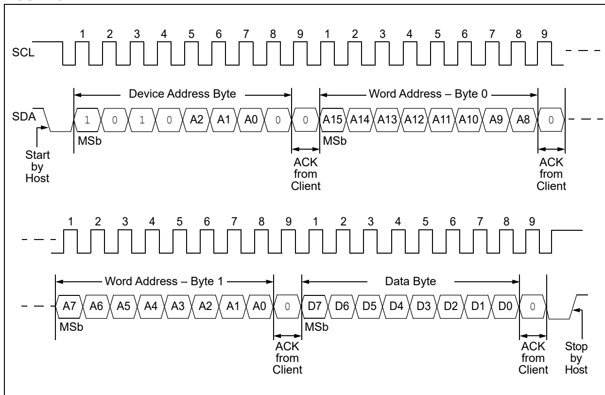
FIGURE 6-1: BYTE WRITE
