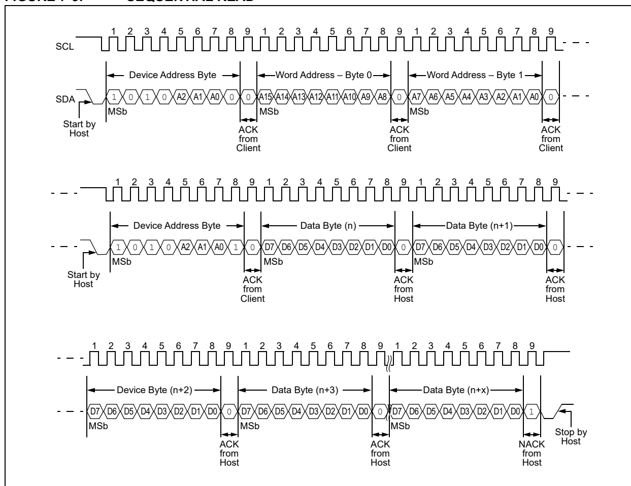
FIGURE 7-3: SEQUENTIAL READ
