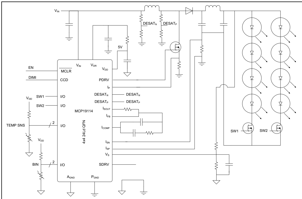
FIGURE 1-3: MCP19114 BOOST QUASI-RESONANT APPLICATION DIAGRAM
