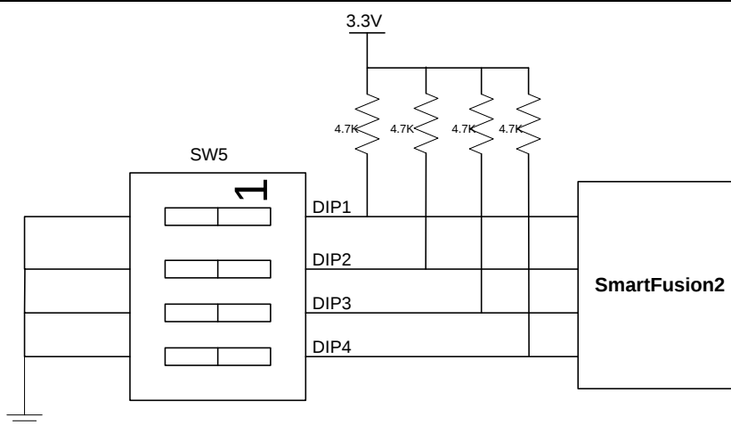
Figure 17 SPST Interface
