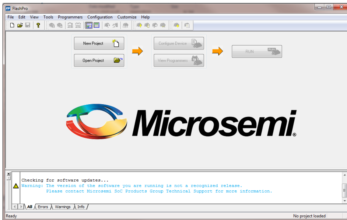
Figure 68 FlashPro Window
