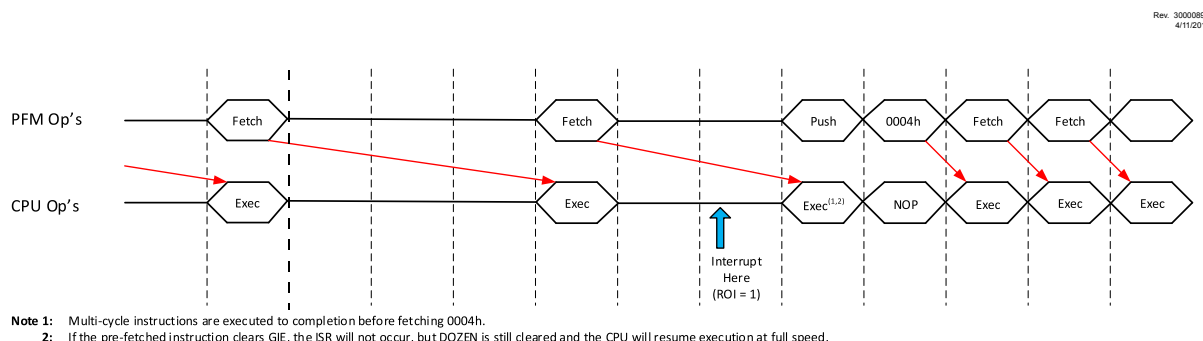
Figure 11-1. DOZE MODE OPERATION EXAMPLE (DOZE<2:0> = 001, 1:4)
