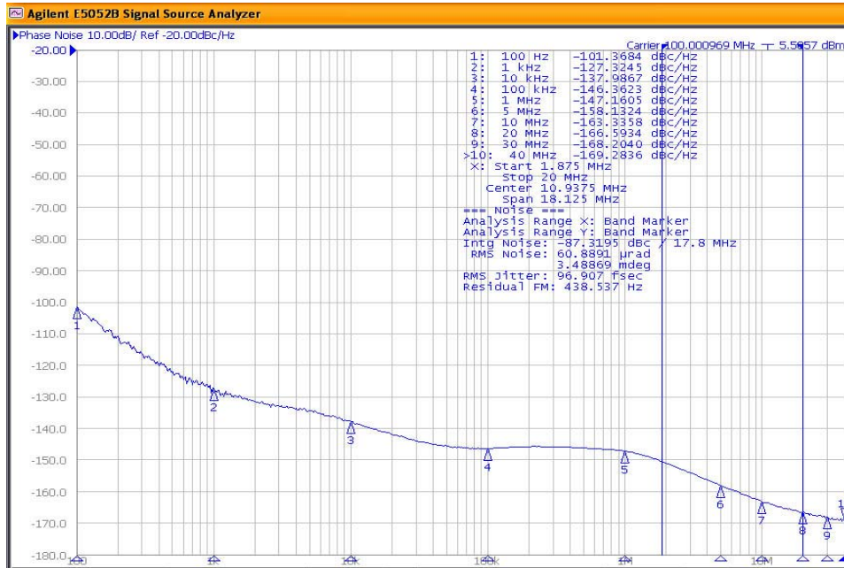
FIGURE 3-7: HCSL Output 100 MHz 1.875 MHz - 20 MHz 97 fs.
