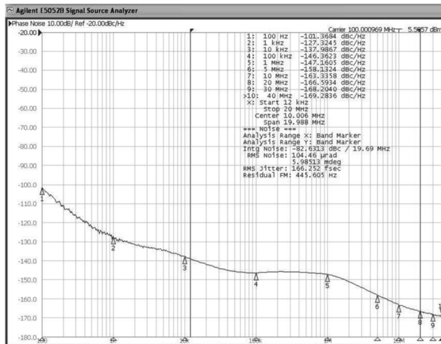
FIGURE 3-8: HCSL Output 100 MHz 12 kHz - 20 MHz 166 fs.
