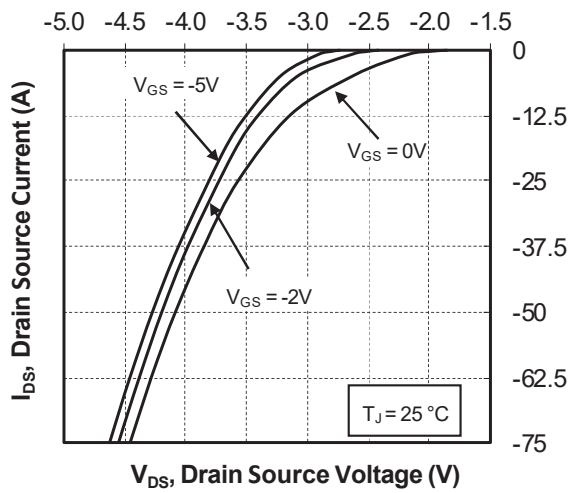
Figure 1-26. Body Diode Characteristics, T_J = 25^\circ\text{C}
