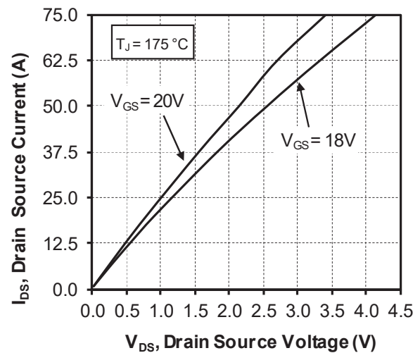
Figure 1-21. Output Characteristics, T_J = 175^\circ\text{C}
