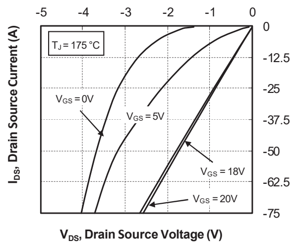
Figure 1-29. 3 rd Quadrant Characteristics, T_J = 175^\circ\text{C}
