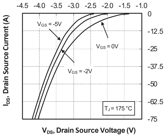
Figure 1-28. Body Diode Characteristics, T_J = 175^\circ\text{C}
