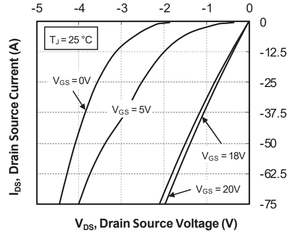
Figure 1-27. 3 rd Quadrant Characteristics, T_J = 25^\circ\text{C}
