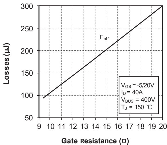
Figure 1-32. Turn-Off Energy vs. Rg
