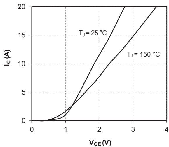
Figure 1-38. Output Characteristics ( V_{GE} = 15V )
