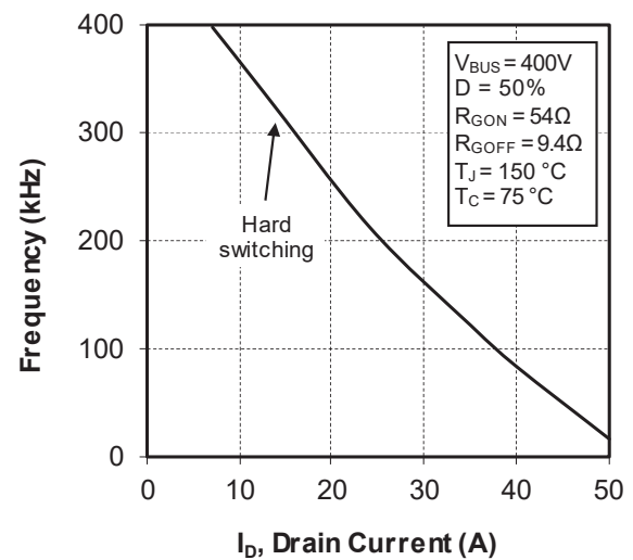
Figure 1-33. Operating Frequency vs. Drain Current
