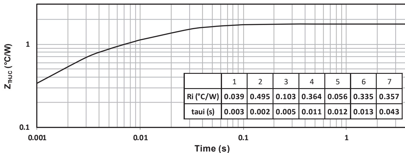
Figure 1-34. Maximum Thermal Impedance
