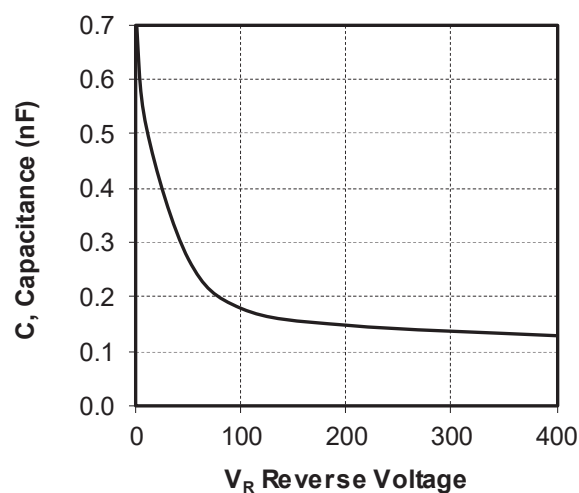
Figure 1-36. Capacitance vs. Reverse Voltage
