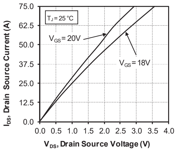
Figure 1-20. Output Characteristics, T_J = 25^\circ\text{C}
