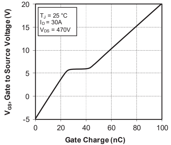
Figure 1-25. Gate Charge vs. Gate Source Voltage
