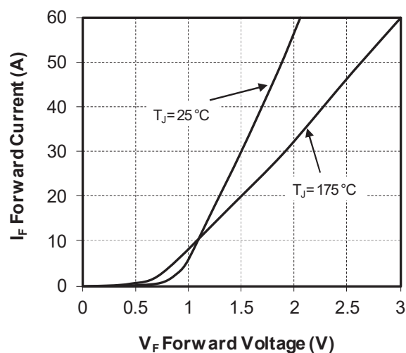
Figure 1-35. Forward Characteristics
