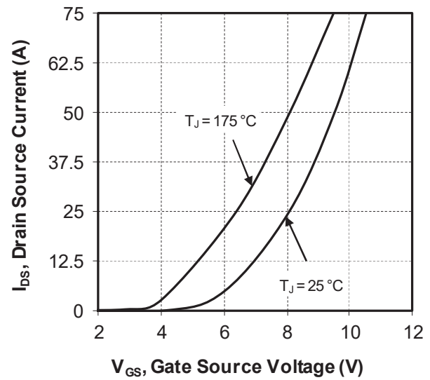
Figure 1-23. Transfer Characteristics
