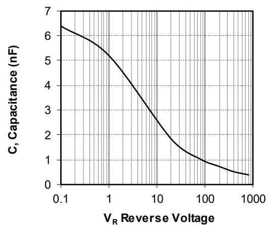
Figure 1-18. Capacitance vs. Reverse Voltage
