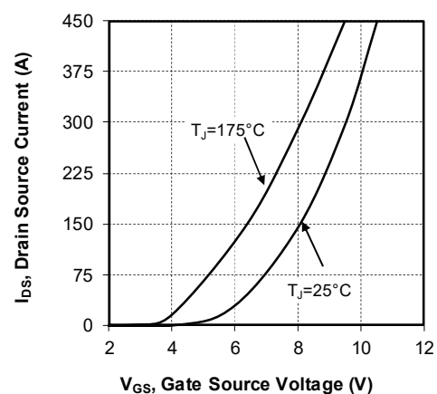
Figure 1-5. Transfer Characteristics
