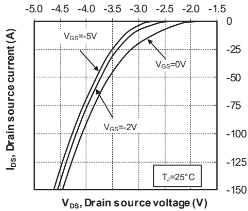
Figure 1-10. Body Diode Characteristics, TJ = 25 °C
