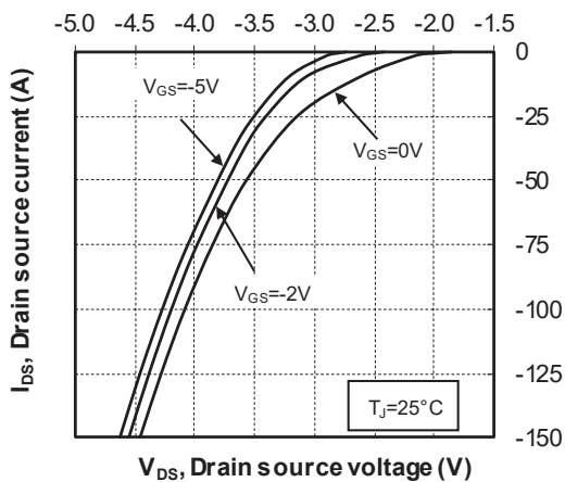
Figure 1-10. Body Diode Characteristics, TJ = 25 °C
