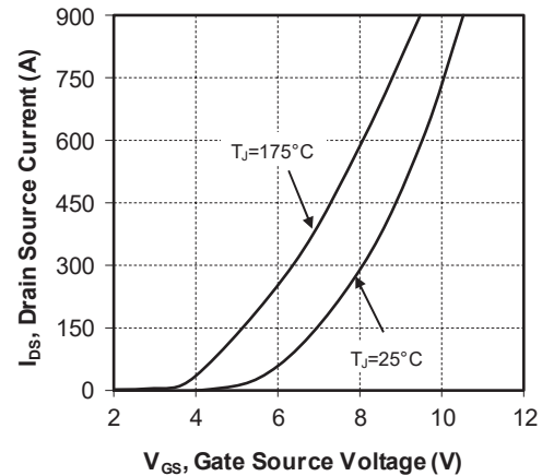
Figure 1-5. Transfer Characteristics
