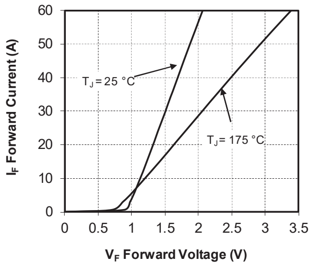
Figure 1-16. Forward Characteristics
