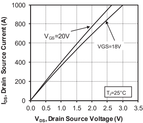
Figure 1-2. Output Characteristics, T_J = 25^\circ\text{C}
