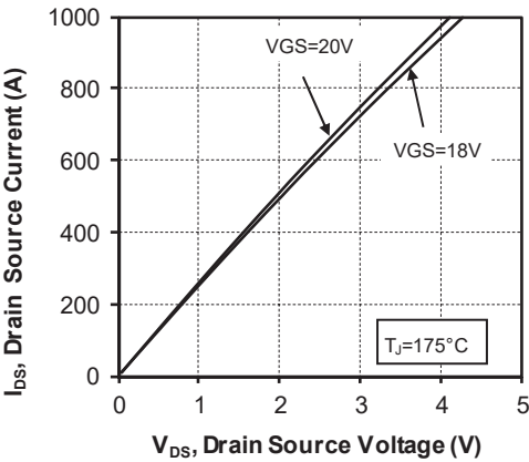
Figure 1-3. Output Characteristics, T_J = 175^\circ\text{C}
