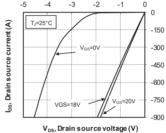
Figure 1-11. 3 rd Quadrant Characteristics, T_J = 25^\circ C
